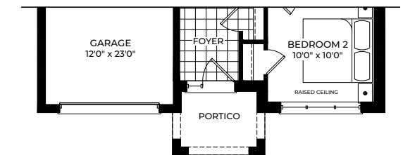
PART. GROUND FLOOR ELEV. B2/OPT. B2
