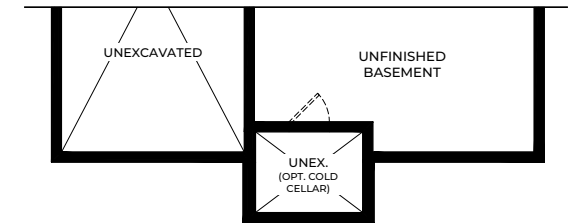
PART. BASEMENT ELEV. B2
